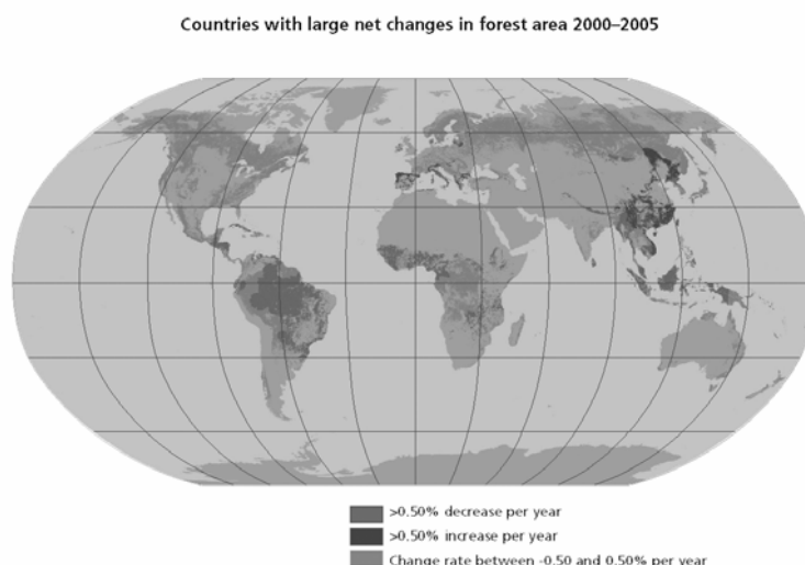
Figure 1.3: Changes in forest area worldwide 2000 - 2005 (FAO 2006)
