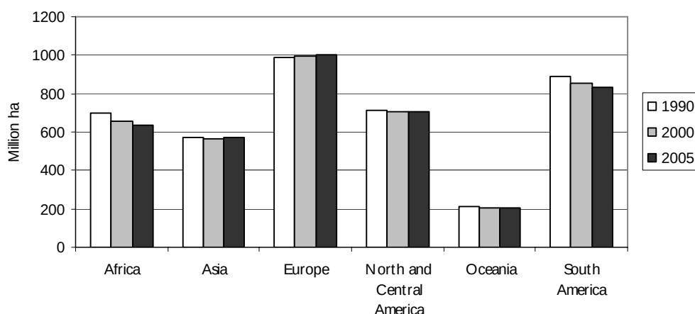
Figure 1.2: Trends in forest area by region 8 1990-2005 (FAO 2006)
