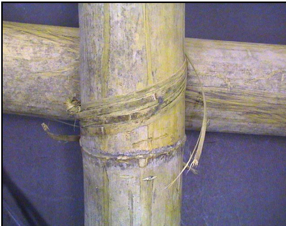
Figure 4.5 Strip splitting
