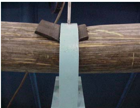
c) Typical failure mode - Local crushing
