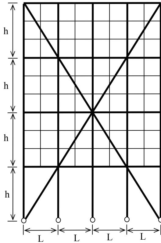
Figure 5.1 Typical configuration of SLBS and DLBS
