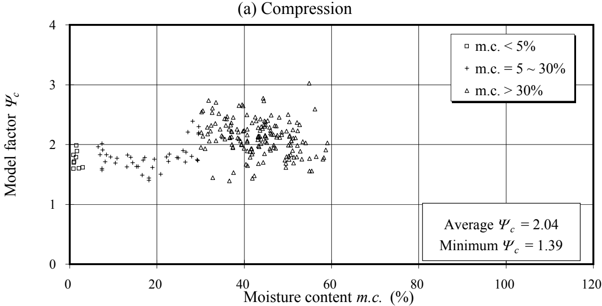
Figure 2.10 Variation of model factors of Mao Jue against moisture content
