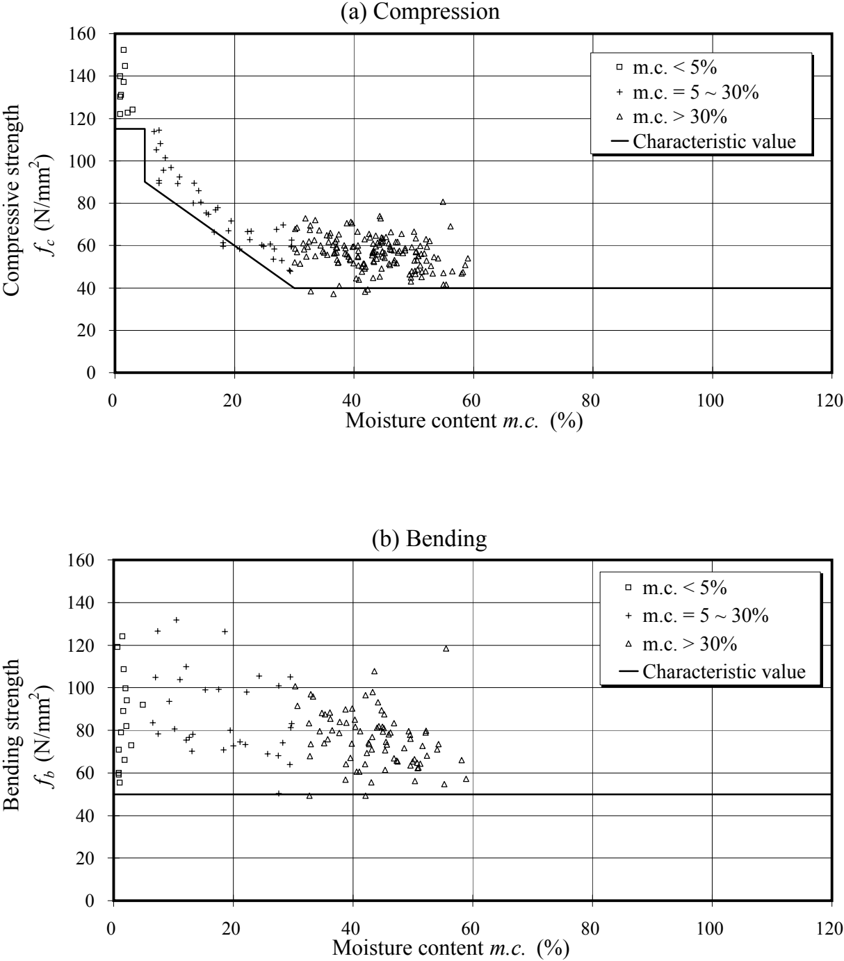
Figure 2.6 Variation of mechanical properties of Mao Jue against moisture content
