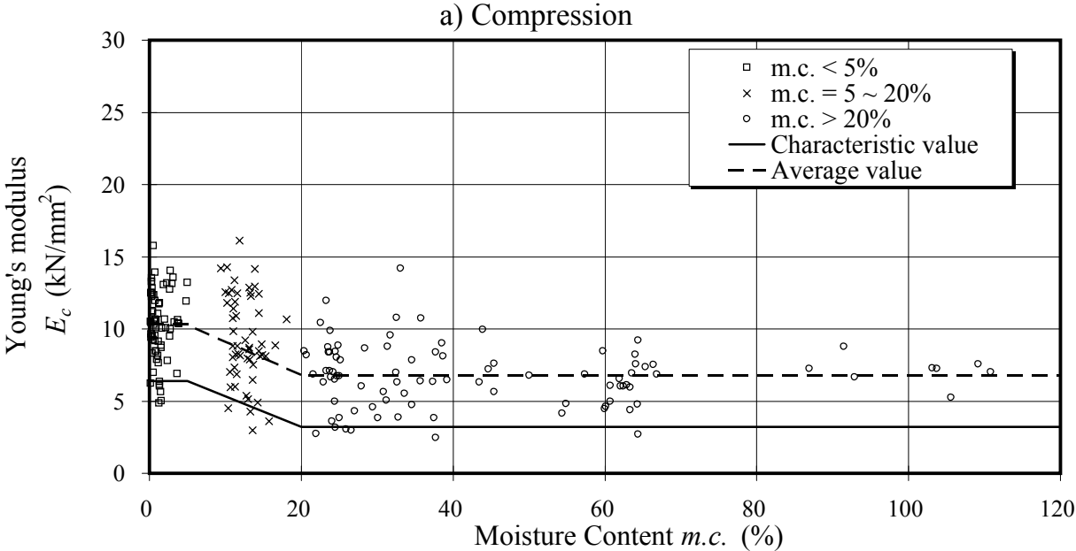
Figure 2.7 Variation of mechanical properties of Kao Jue against moisture content
