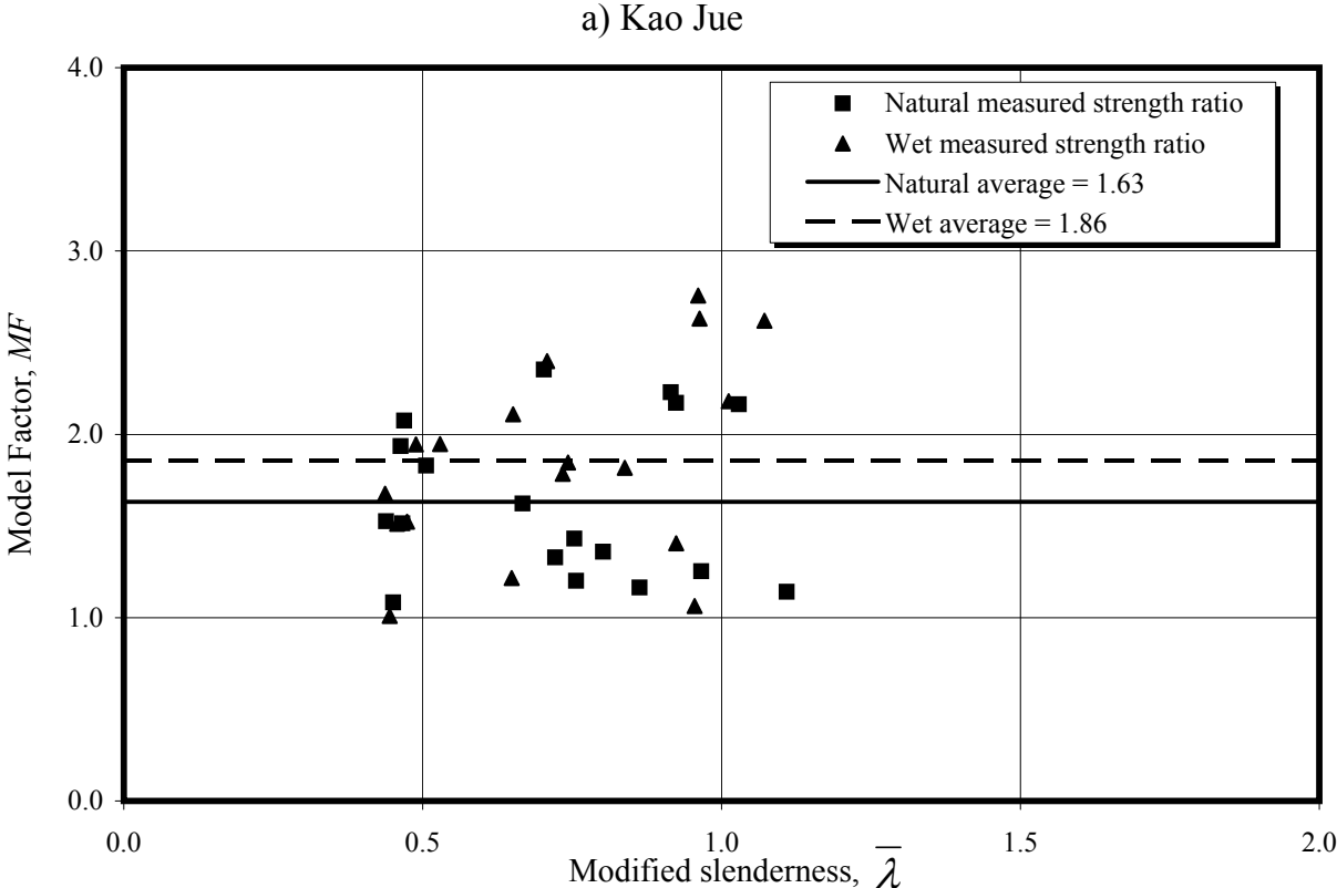
Figure 3.5 Model factors for column buckling design
