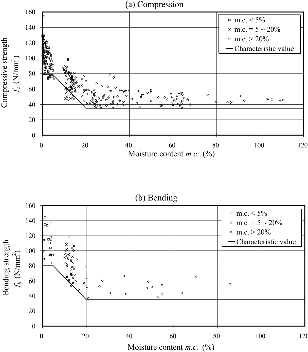
Figure 2.5 Variation of mechanical properties of Kao Jue against moisture content
