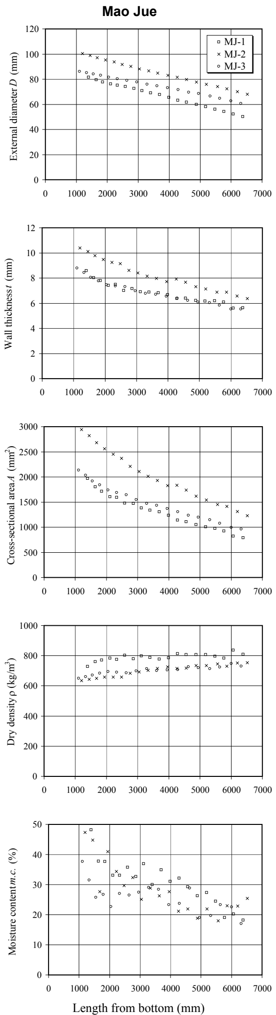
Figure 2.2 Variation of physical properties along length of bamboo culms
