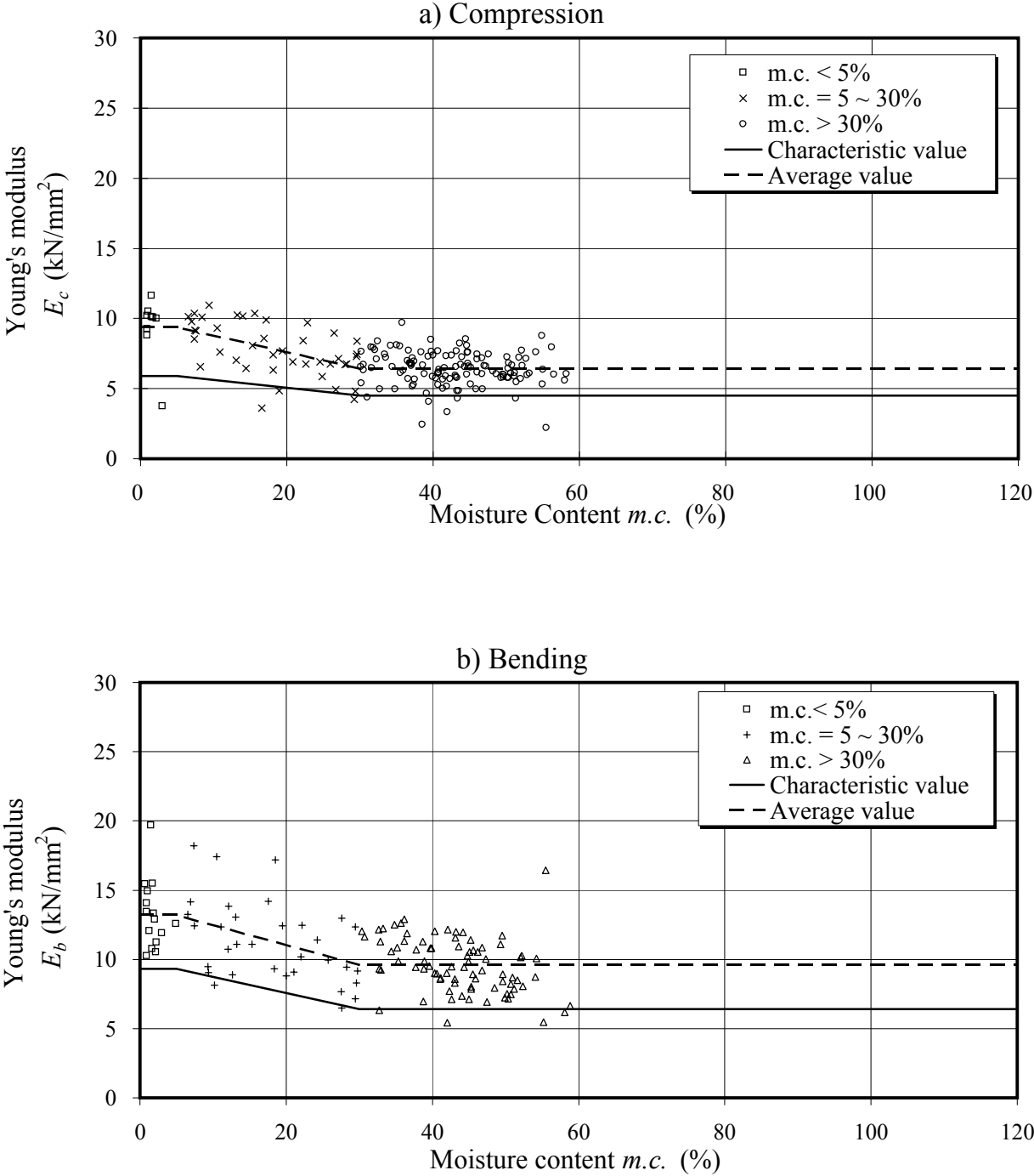
Figure 2.8 Variation of mechanical properties of Mao Jue against moisture content
