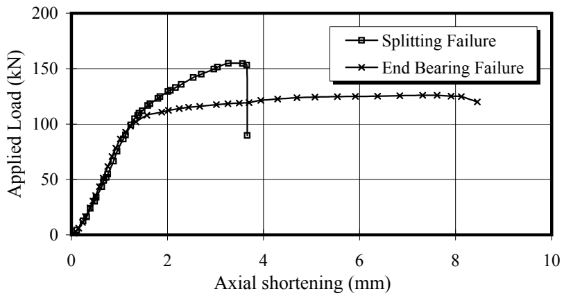
b) Load deflection curves
