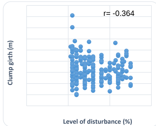
Figure 13. Correlation analysis of the level of disturbance and clump girth
