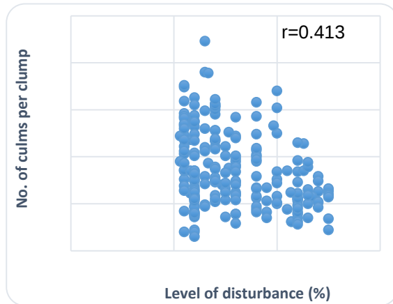
Figure 14. Correlation analysis of the level of disturbance and number of culms per clump
