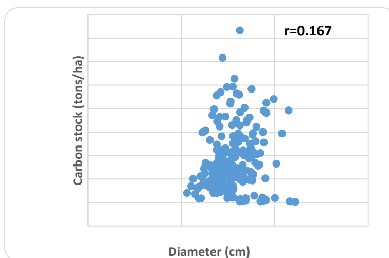
Figure 19. Relationship between culm diameter and carbon stock
