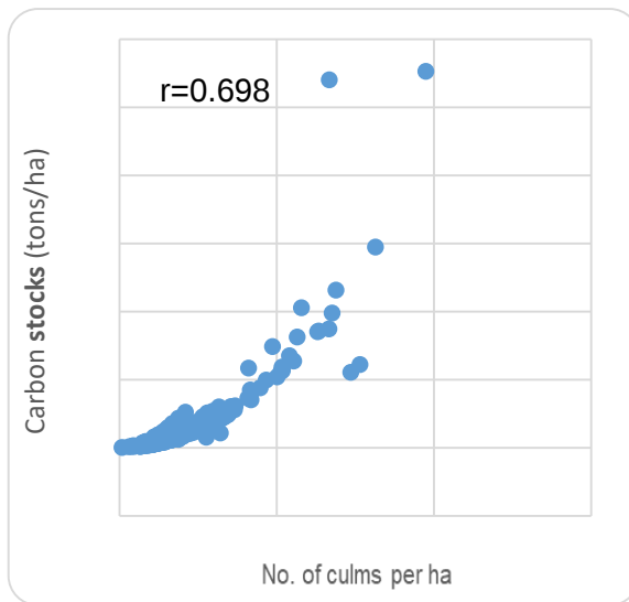
Figure 15. Figure relationship between number of culms per hectare
