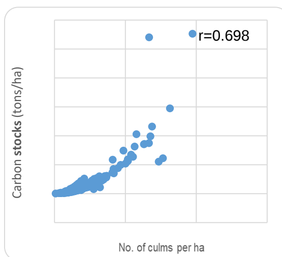
Figure 17. Relationship between number of basal area culms per hectare and carbon (tons/ha)
