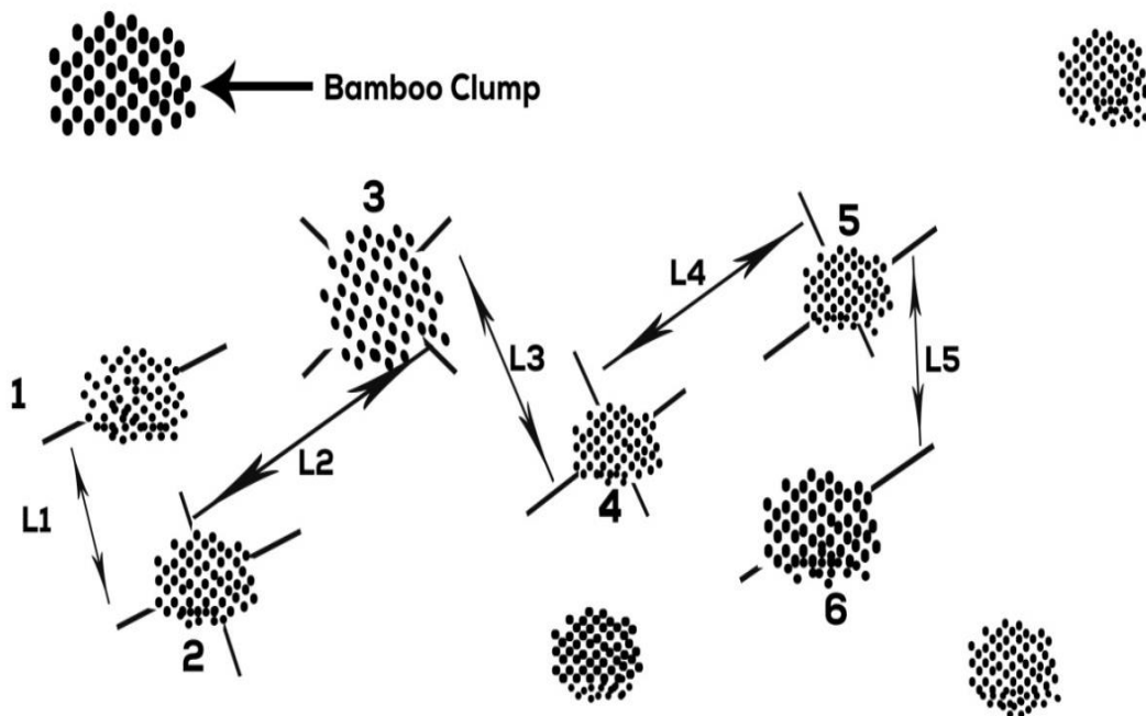
Figure 4. Systematic selection of clumps for measurement
