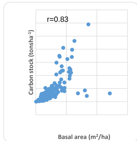
Figure 16. Figure association between basal area (m²/ha) and carbon stocks (tons/ha)
