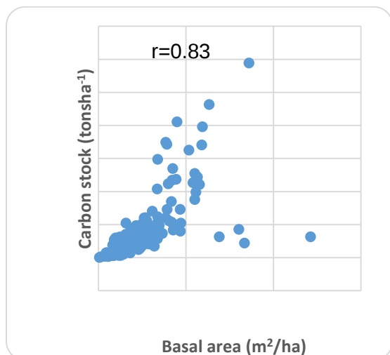
Figure 18. Association between m^2/ha and carbon stocks
