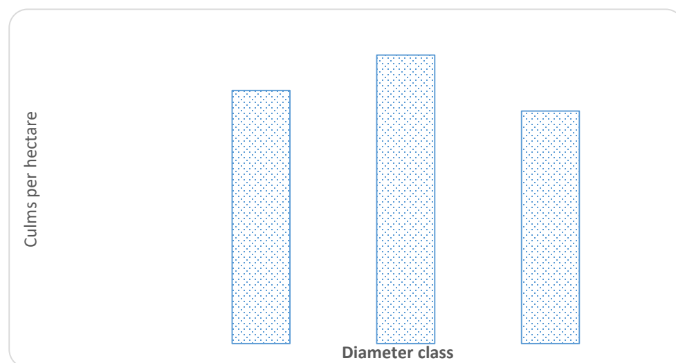
Figure 11. Diameter distribution of culms per hectare
